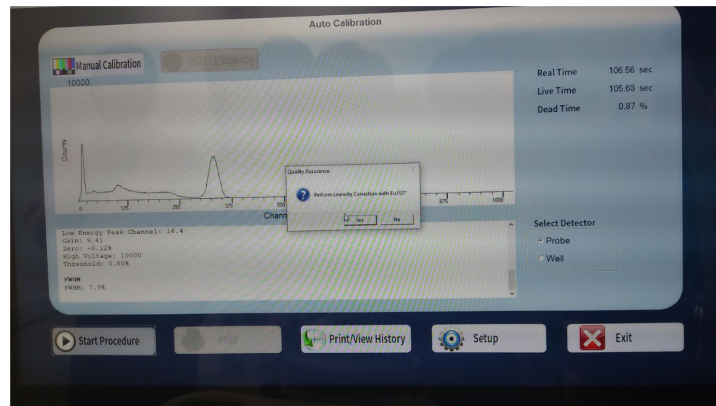
Figure 5: Calibration of thyroid uptake measurement unit using ^{137}\text{Cs} source.
