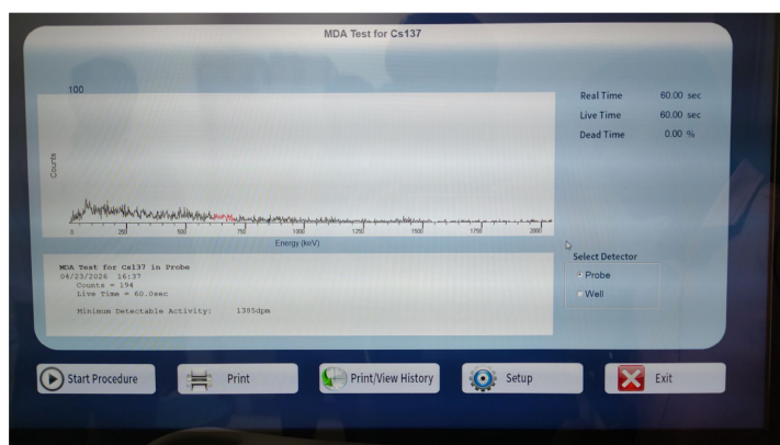
Figure 9: MDA test of the system using Cs137 source.
