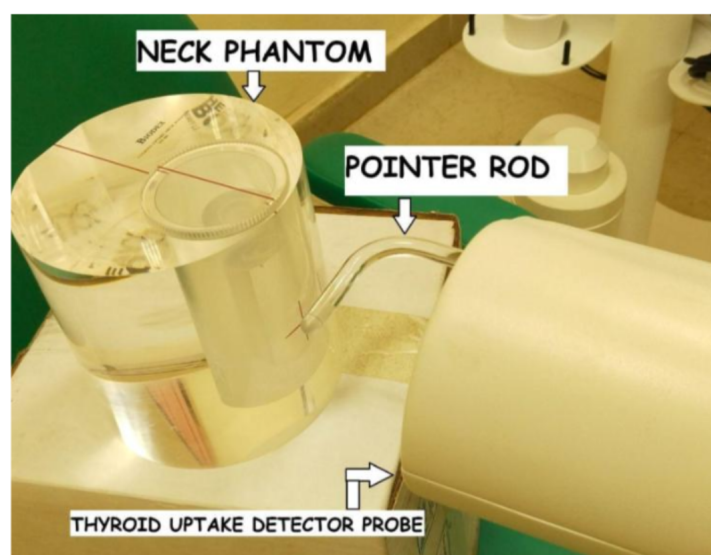
Figure 10: Standard dose measurement setup using neck phantom and thyroid probe at 25cm
