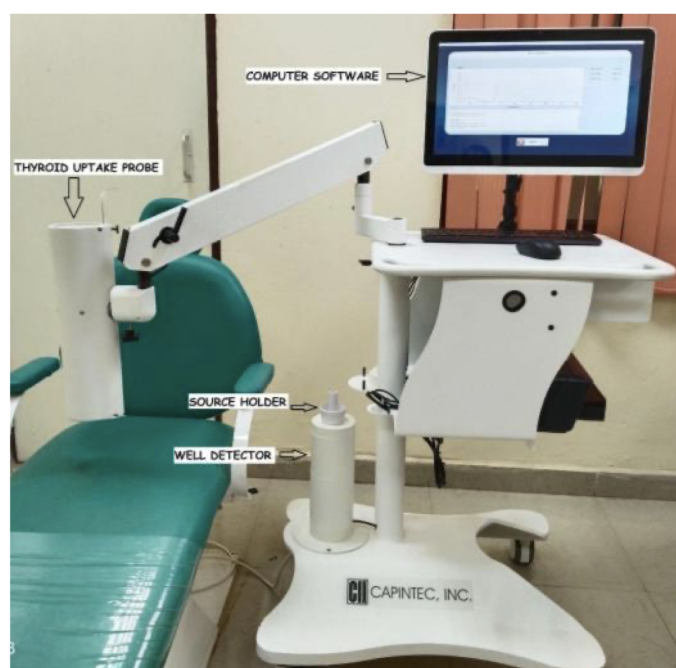
Figure 3: The CAPTUS 4000e Thyroid Uptake System.
