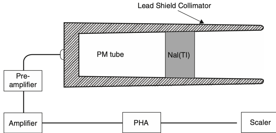
Figure 2: Schematic representation of a thyroid probe system, illustrating the NaI(Tl) scintillation crystal, photomultiplier tube, lead collimator, and associated electronic processing units. The collimator restricts the field of view to the thyroid region, while the scintillation crystal converts incident gamma photons into visible light, which is then amplified by the PMT for quantitative analysis.
